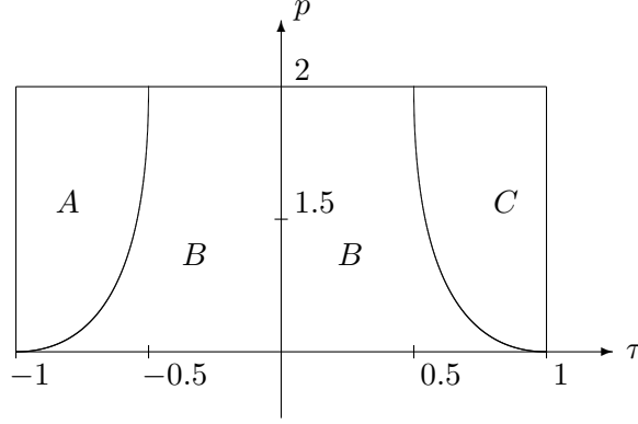
FIGURE 10. Splitting [-1, 1] \times (1, 2) in the (\tau \times p) -plane into three regions A, B and C . The curves separating regions A, B and C are where M_{y_2y_2} = 0 in Case (2 2 ).
