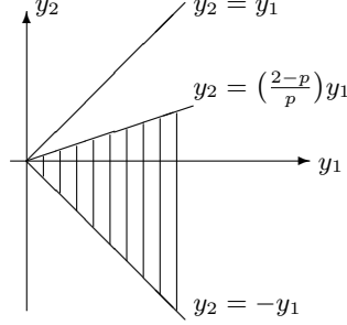
FIGURE 9. Range of characteristics in Case (3 2 ) for 1 < p < 2 .
