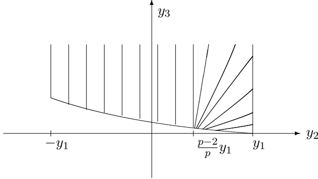
FIGURE 5. Characteristics of Bellman candidate for 2 < p < \infty
