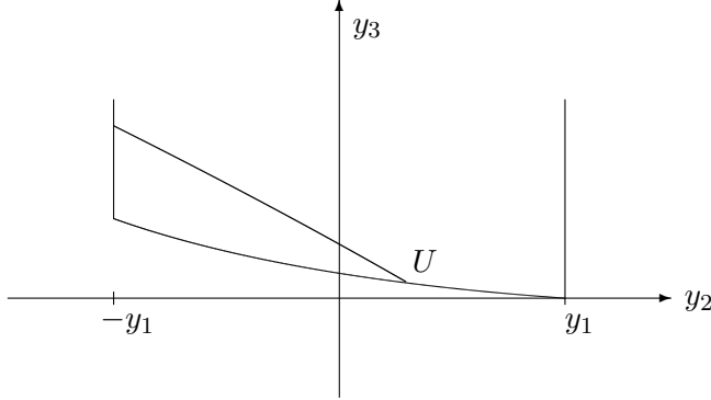
FIGURE 8. Sample characteristic of Monge–Ampère solution in Case (3 2 )
