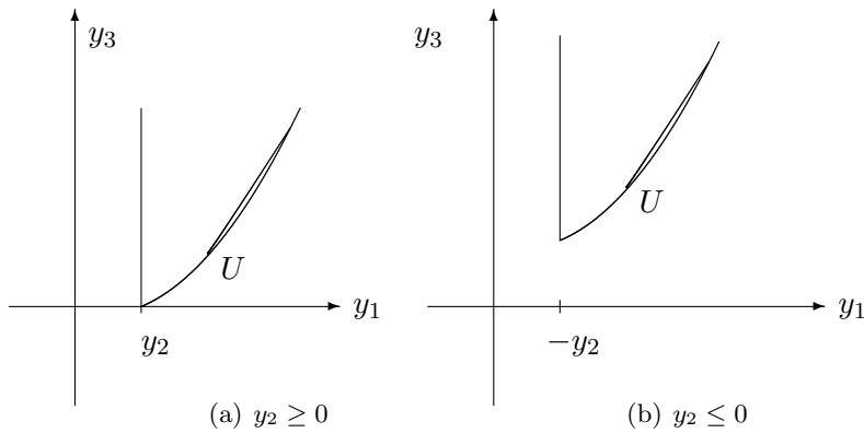
FIGURE 12. Characteristic of solution in Case (4 1 ).
