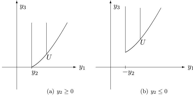
FIGURE 3. Sample characteristic of Monge–Ampère solution in Case (2 1 )
