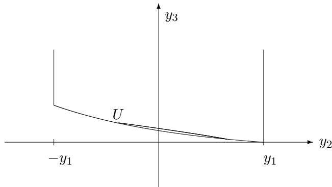
FIGURE 13. Characteristic for the solution from Case (4 2 )
