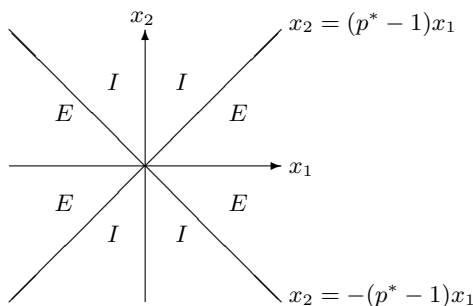
FIGURE 7. Location of Implicit (I) and Explicit (E) part of B_\tau for 2 \leq p < \infty .
