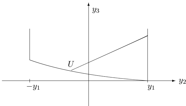
FIGURE 1. Sample characteristic of solution from Case (1_2)
