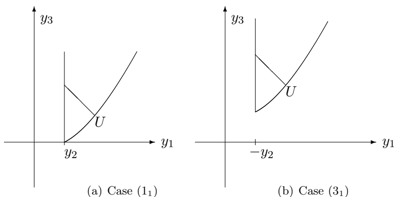
FIGURE 11. Sample characteristic for Monge–Ampère solution in Cases (1 1 ) and (3 1 )
