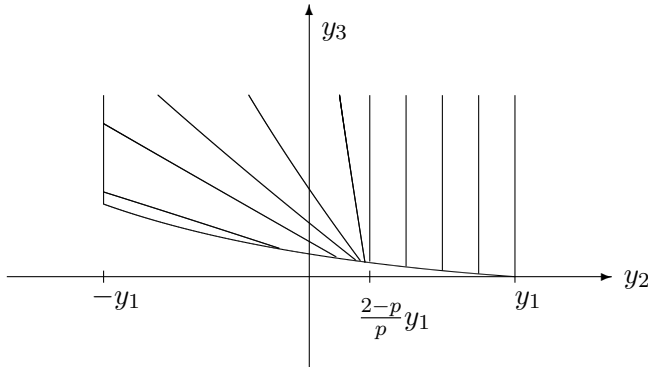
FIGURE 6. Characteristics of Bellman candidate for 1 < p < 2 and |\tau| \leq \frac{1}{2} .
