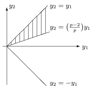
FIGURE 2. Sector for characteristics in Case (1 2 ), when p > 2 .
