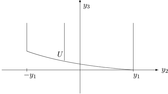
FIGURE 4. Sample characteristic of Monge–Ampère solution for Case (2 2 )
